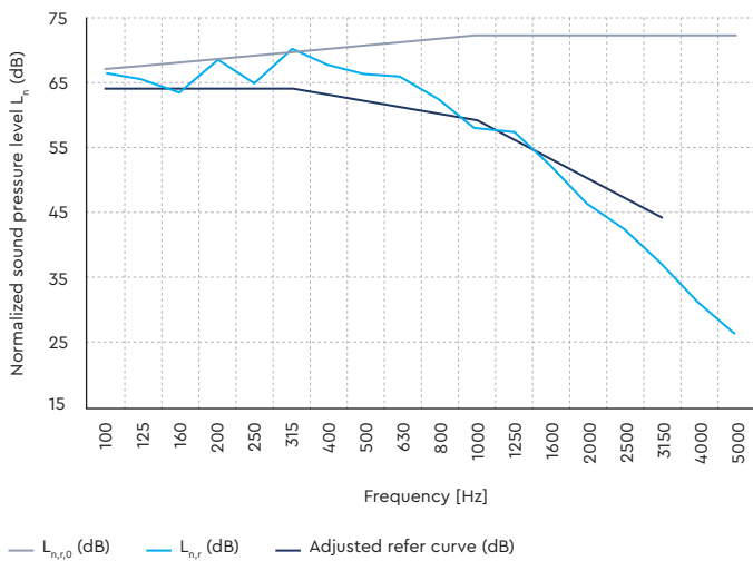
Impact Insulation (IS) · Wood floor (21mm) · T66 (3mm) · Glued
