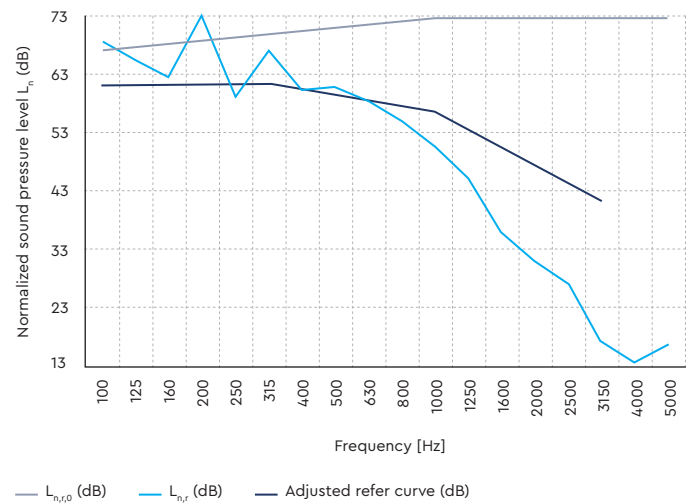
Impact Insulation (IS) · Wood floor (12mm) · T66 (3mm) · Floating
