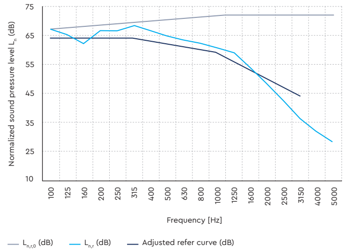
Impact Insulation (IS) · Ceramic floor (9.5mm) · T66 (3mm) · Glued
