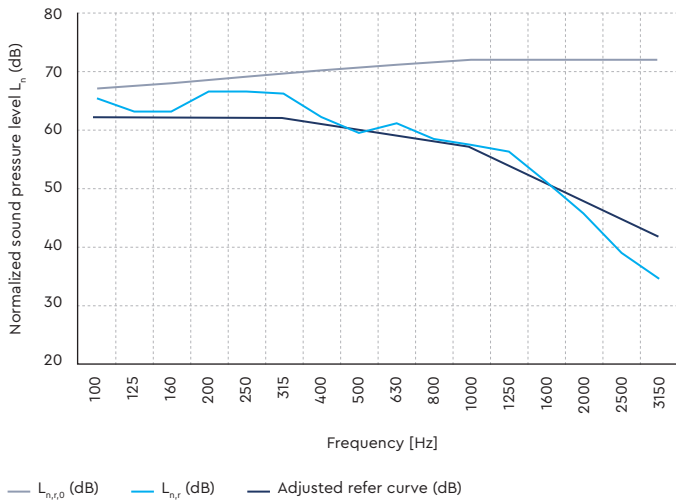
Impact Insulation (IS) · Ceramic floor (9mm) · T66 (4.5mm) · Glued
