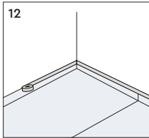
The barrier must be installed directly onto the surface of the subfloor. Use a sealing tape to seal the rows securely together.
