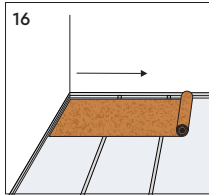
The underlayment should be installed in a perpendicular direction to the final floor, which should always be installed in the direction of natural light incidence in the room.
