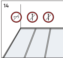
Never mechanically secure the barrier with screws, nails or staples, since this may undermine its effectiveness.
