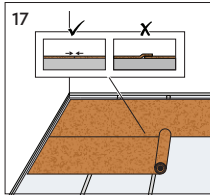
The underlayment must cover the entire area without any gaps nor overlaps.
