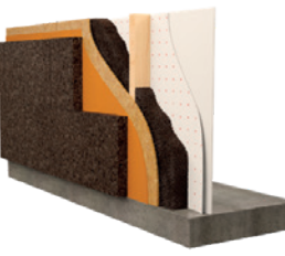
External walls Exterior cladding over wooden substrate - cork at sight
